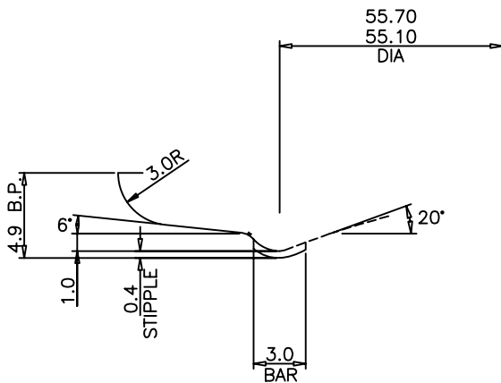
STACKING RING & STIPPLE DETAIL - SCALE 5:1
