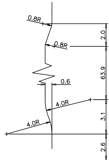
PANEL DETAIL - SCALE 10:1
