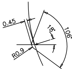
TYPICAL (1.8 DIA) DOT CODE SECTION SCALE 5:1
