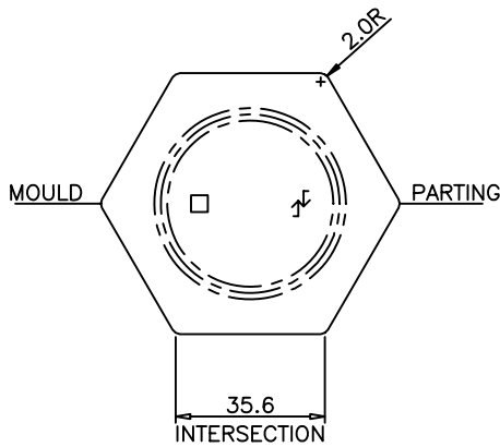
VIEW ON BASE SHOWING EMBOSSED MARKING
