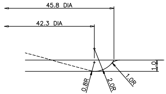
STACKING RING DETAIL SCALE 10:1
